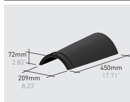
Q02*K | Round ridge / Hip klinker
