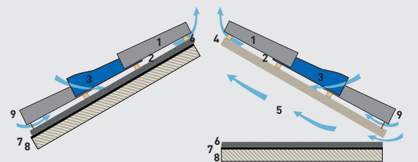
NON-VENTILATED ROOF
